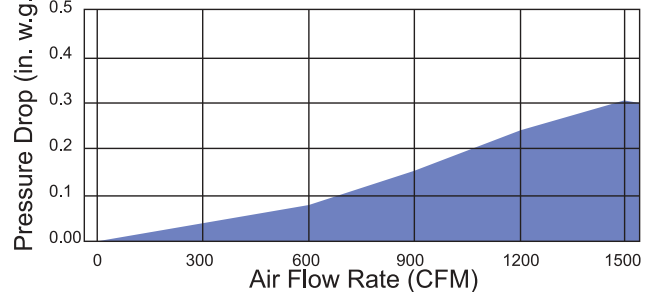
Initial Resistance vs. Air Flow Rate
