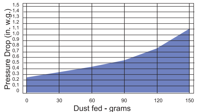
Dust Fed vs. Resistance
